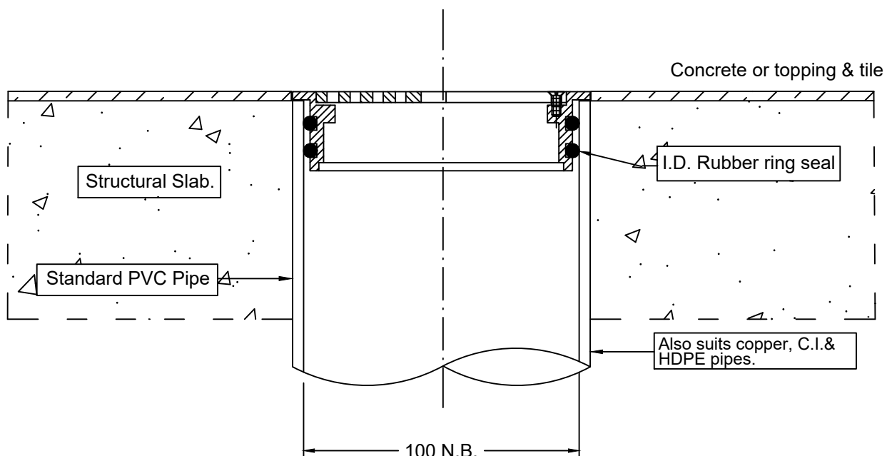
Typical Application
