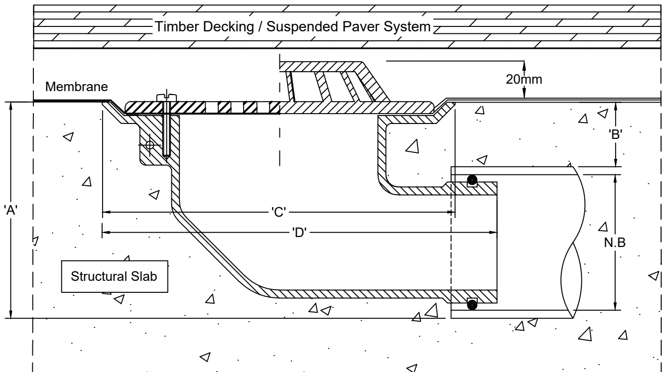
Typical Application
