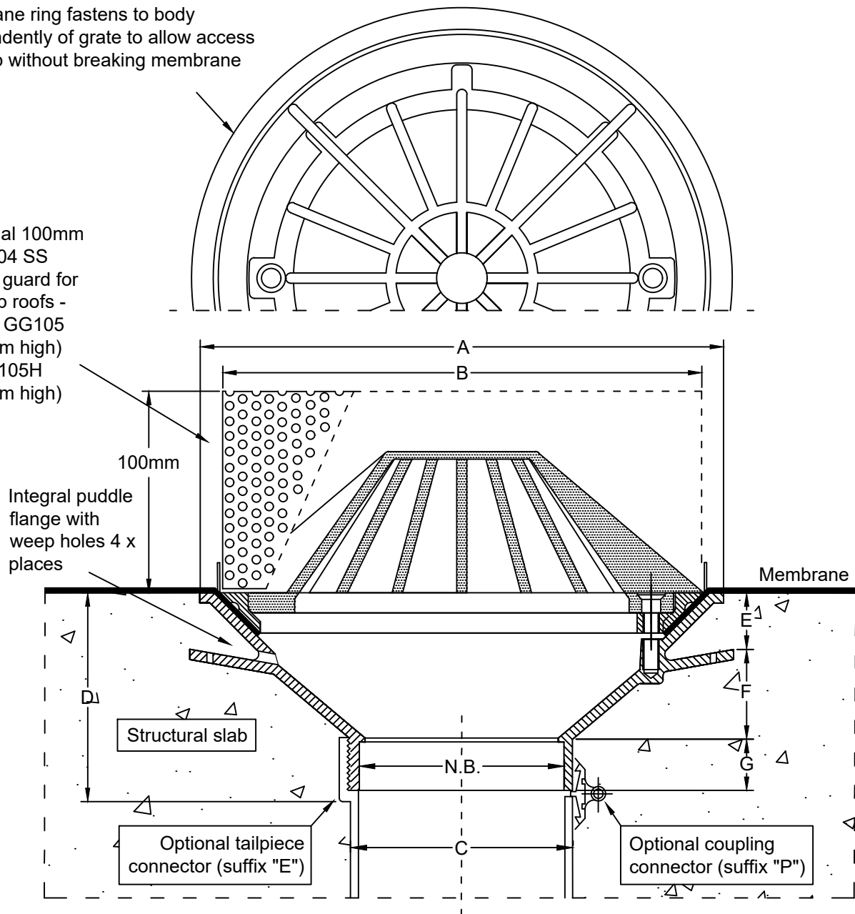
Dimensions (mm)
