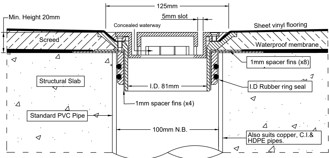
Typical Application
